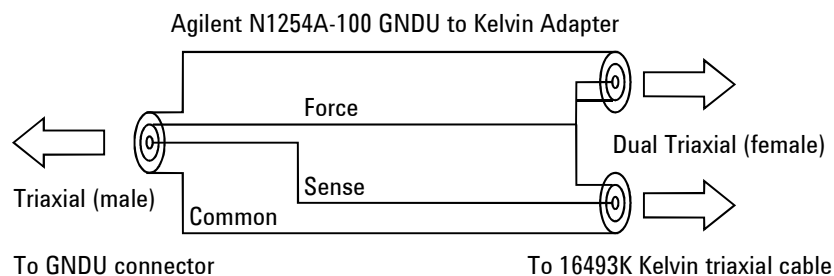
Figure 3-6 Agilent N1254A-100 GNDU-Kelvin アダプタ
