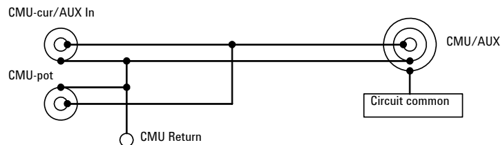
Setup 2: AUX On ( CMU/AUX input to ASU output )
